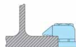
PARALLEL FLANGE 16mm thick at edge. Slight gap under nose, full contact at skirt.
