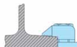
TAPER FLANGE 16mm thick at edge. Full contact at nose and skirt.
